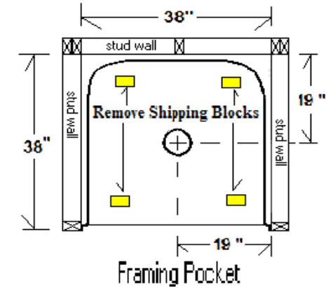
Drawing A - 1 Model 11383834 Shower Framing Pocket
