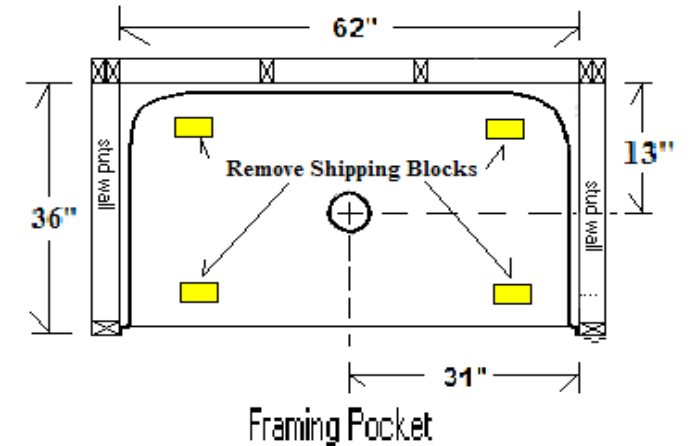
Drawing A - 2 – Model 11623634 Shower Framing Pocket
